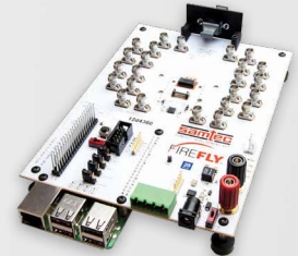
28 Gbps FireFly™ Kit
