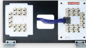
Si-Fly™ Low Profile Cable System (CPC/CPI)
