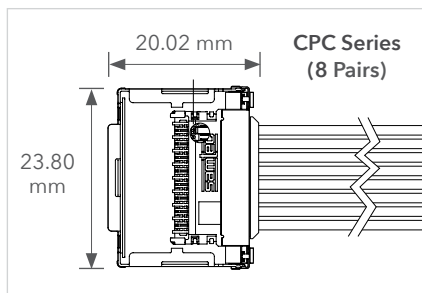
Incredibly low 3.8 mm mated profile
