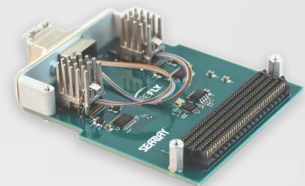
14 Gbps FireFly™ FMC Kit
