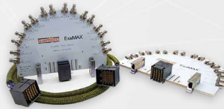
ExaMAX® Backplane Cable System (EBCM/EBTF-RA)
