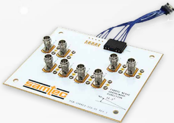
FireFly™ Copper Micro Flyover System™ (ECUE/UEC5-2/UCC8)
