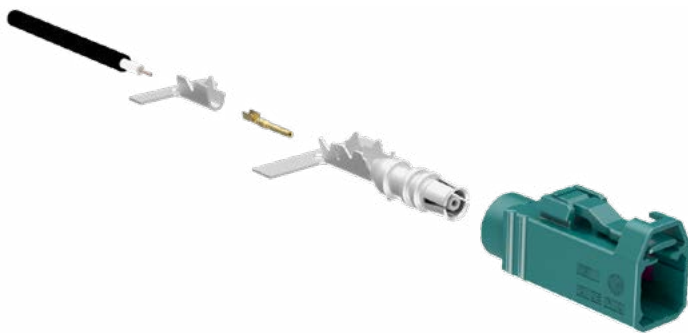
Cable SF support sleeve SF center contact SF connector body Plastic housing
