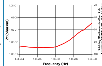
Transfer Impedance Measurement (Size 11)
