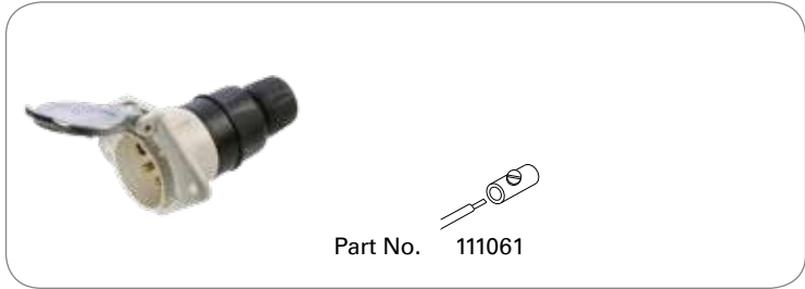
7P/24V Plug (ISO 3731 - Type S)
