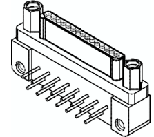
Single Row Micro Sizes 4 thru 25 Page M-129
