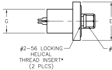
SOLDER CUP OR PIGTAIL TERMINATION (PLUG WITH SOLDER CUP TERMINATION SHOWN)
